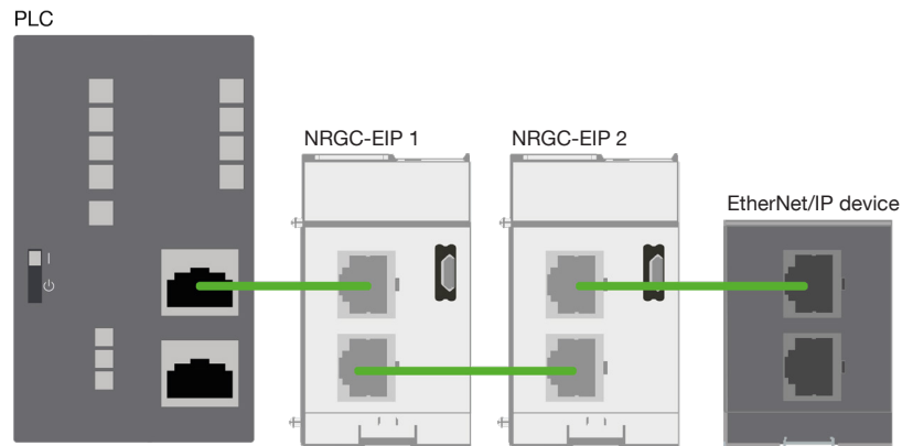
Fig. 3 Example of a line configuration of the NRG-EIP with other EtherNet/IP devices and controller
