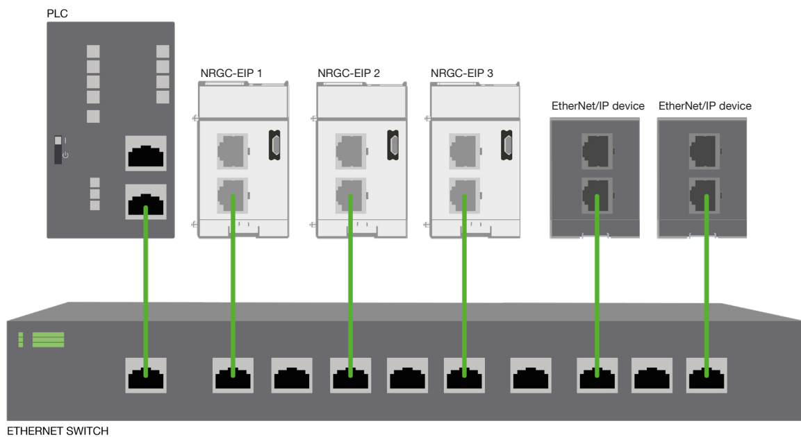
Fig. 4 Example of a star configuration of the NRG-EIP with other EtherNet/IP devices and controller
