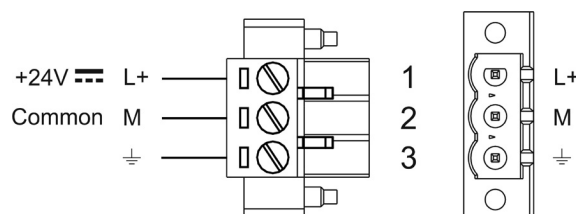
Fig. 2 Power supply
