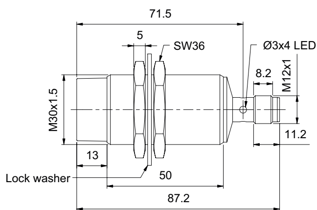
Fig. 24 Long body, non-flush version, plug
