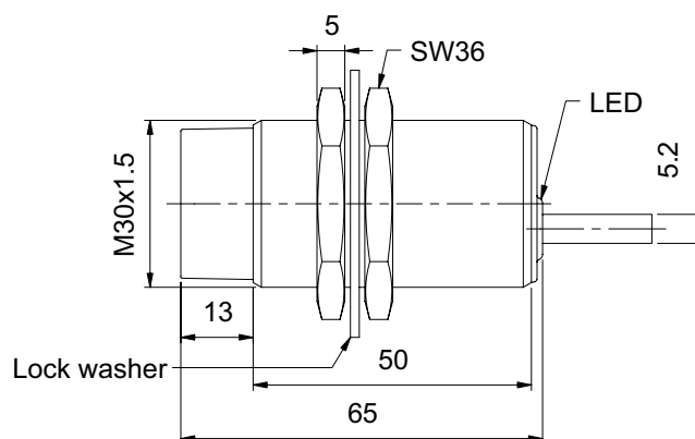
Fig. 22 Long body, non-flush version, cable
